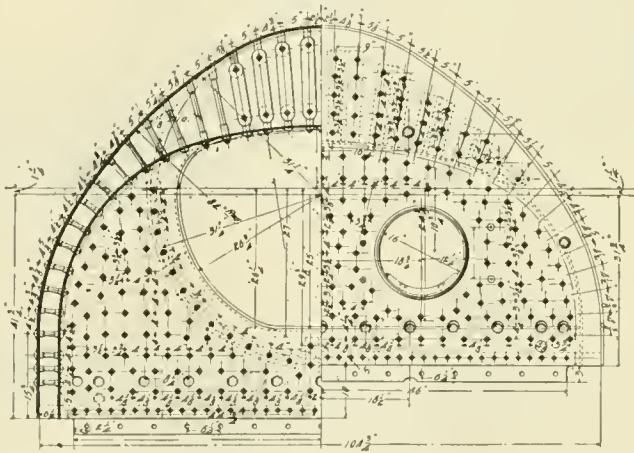
FIREBOX OF JERSEY CENTRAL'S ATLANTIC LOCOMOTIVE.
